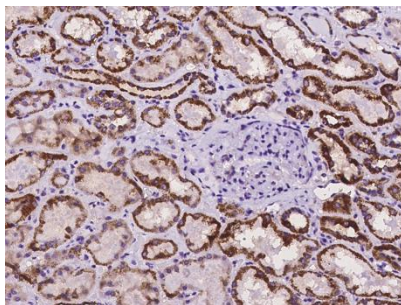
Immunohistochemical staining of human ECHDC2 in human kidney with rabbit polyclonal antibody at 1:100 dilution, formalin-fixed paraffin embedded sections.
