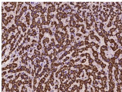
Immunohistochemical staining of human ECHDC2 in human liver with rabbit polyclonal antibody at 1:100 dilution, formalin-fixed paraffin embedded sections.
